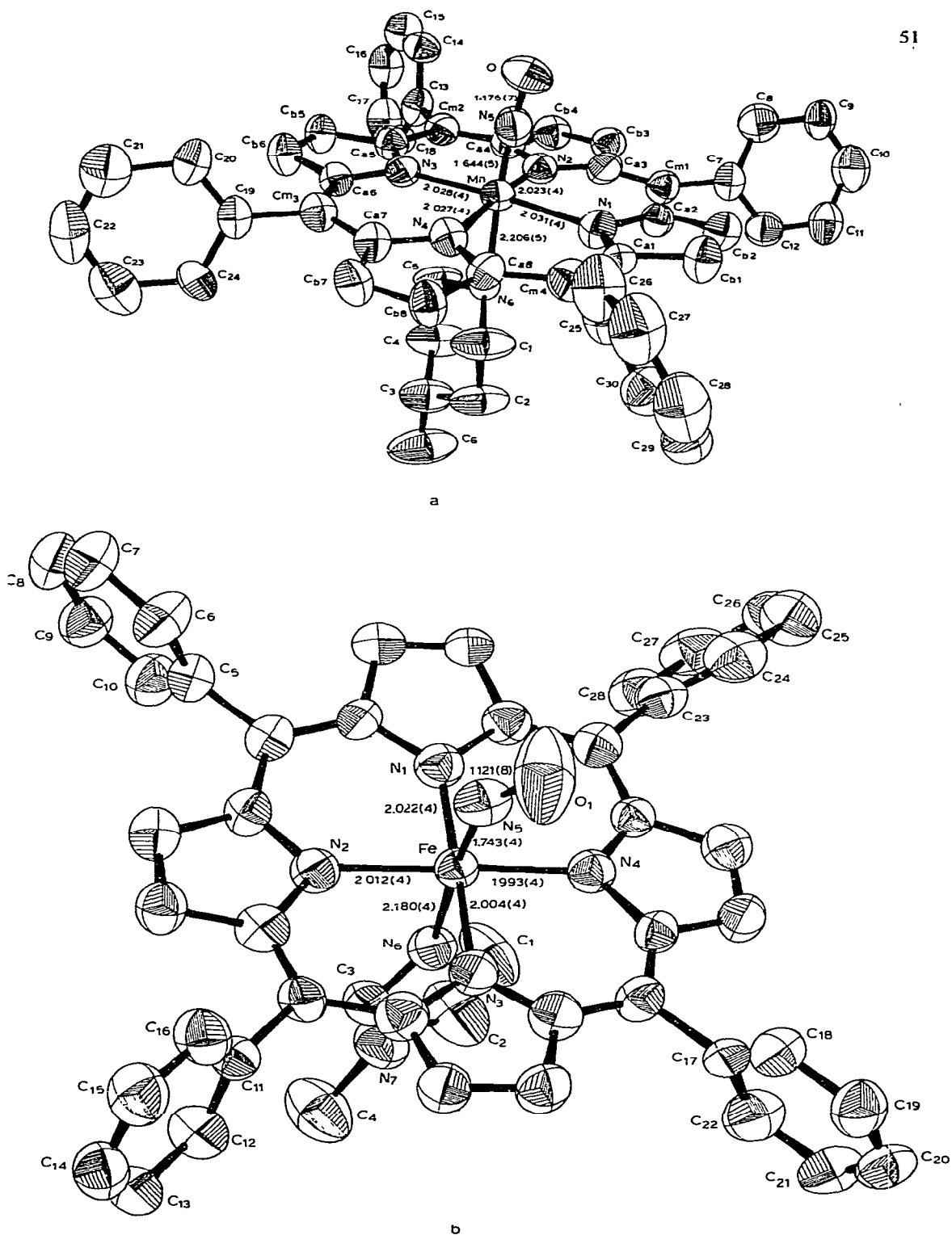
Fig. 12. Computer drawing of the molecules (a) Mn(TPP)NO(4Me-Pip) and (b) Fe(TPP)NO(NMe-Im) from refs. 69 and 73, respectively.
