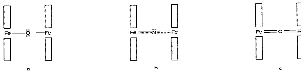
Fig. 23. Schematic representation of (a) \mu -oxo, (b) \mu -nitrido and (c) \mu -carbido complexes.
