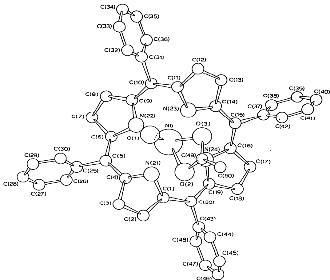
Fig. 19. Computer drawing of the molecule Nb(TPP)O(AcO) from ref. 137.
