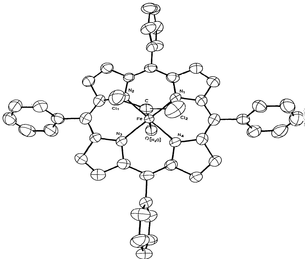
Fig. 8. Computer drawing of the molecule \text{Fe(TPP)CCl}_2(\text{H}_2\text{O}) from ref. 41.
