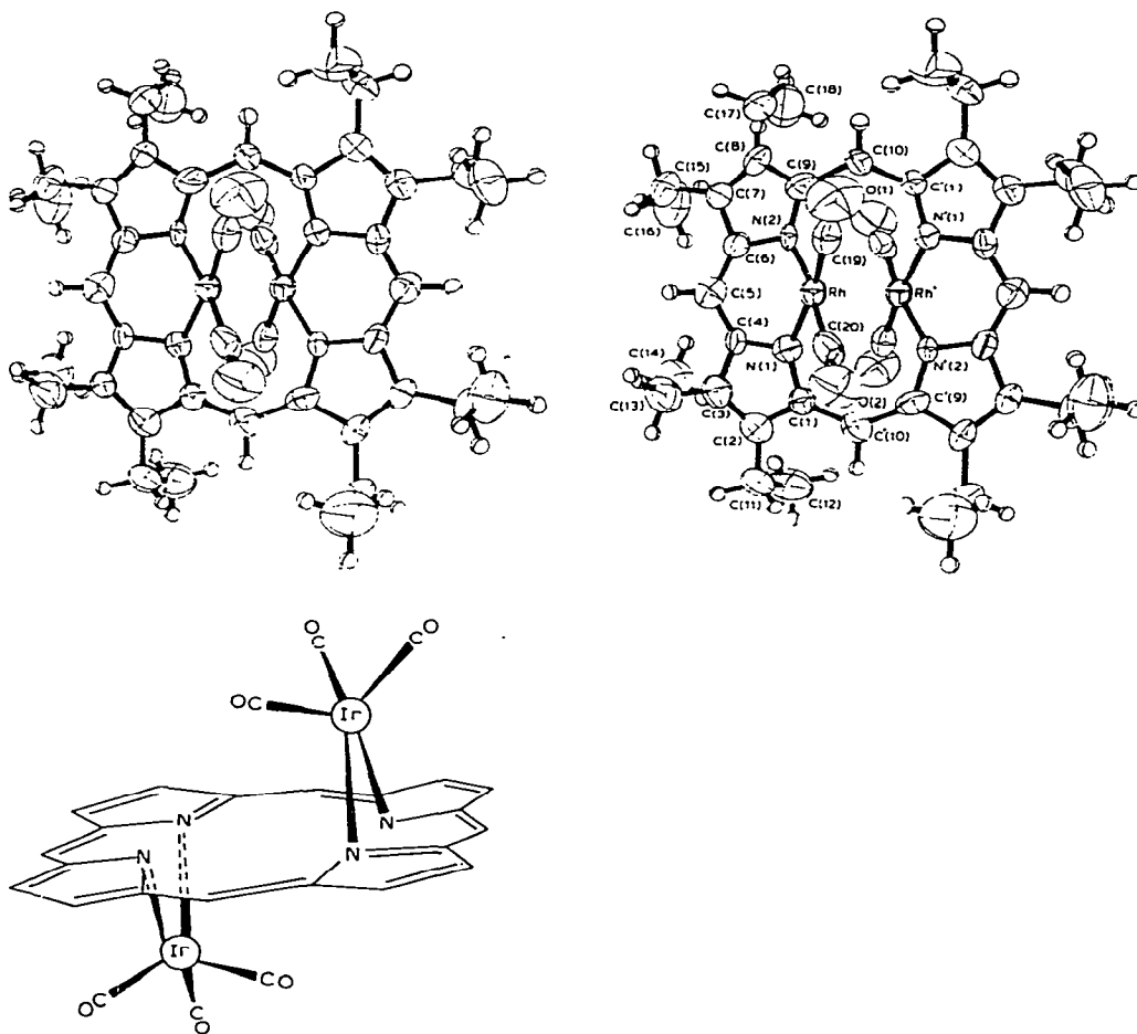
Fig. 7. Computer drawing of the molecule of [Rh(CO)_2]_2(OEP) from ref. 44, and proposed structure for [Ir(CO)_3]_2(OEP) .
