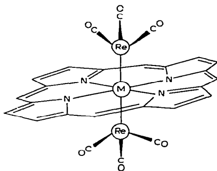
Fig. 26. Schematic representation of the metal-metal bonding in porphyrin complexes.
