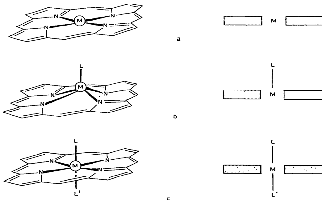
Fig. 1. Common porphyrin coordination geometries, (a) square planar, (b) square pyramidal and (c) octahedral.
