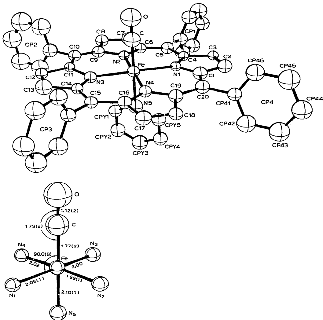
Fig. 2. Computer drawing of the molecule Fe(TPP)CO(Py) and representation of the inner coordination sphere from ref. 29.
