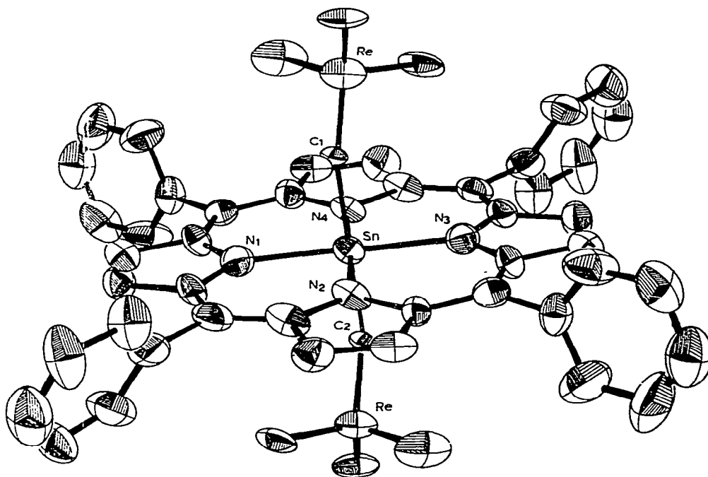
Fig. 27. Computer drawing of the molecule \text{Sn(TPP)[CRe(CO)}_3\text{]}_2 from ref. 162.
