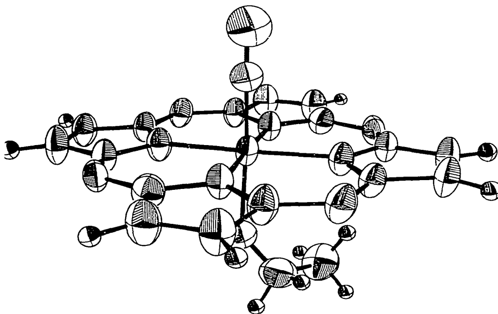
Fig. 4. Computer drawing of the molecule Ru(TPP)CO(EtOH) from ref. 15.
