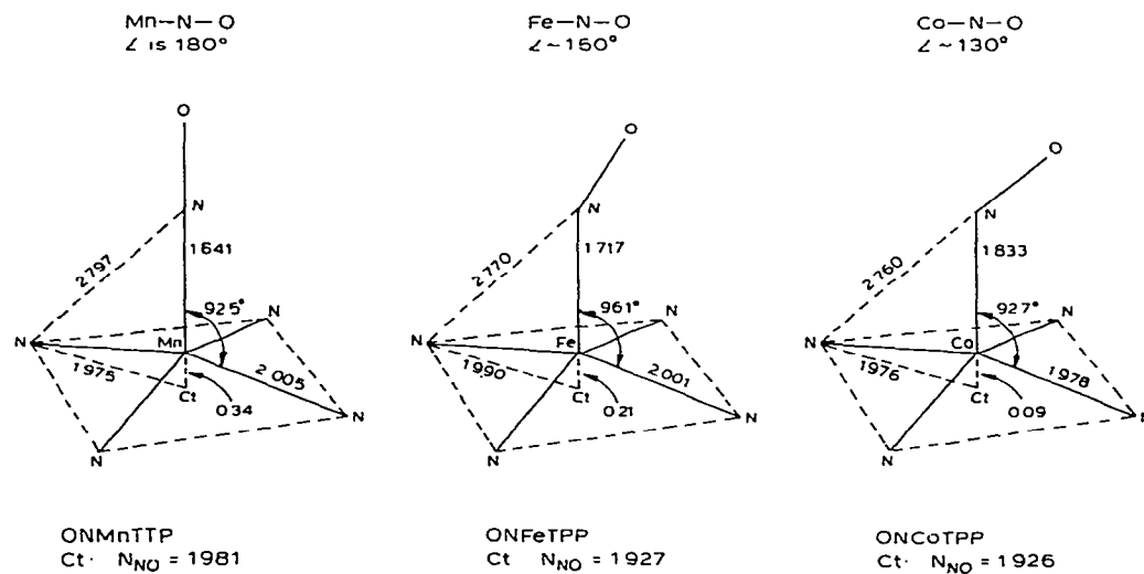
Fig. 11. Comparison of the coordination geometries of the pentacoordinate nitrosyl complexes Mn(TPP)NO, Fe(TPP)NO and Co(TPP)NO from ref. 69.
