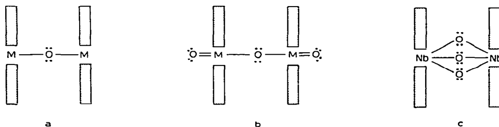
Fig. 20. Examples of \mu -oxo complexes.
