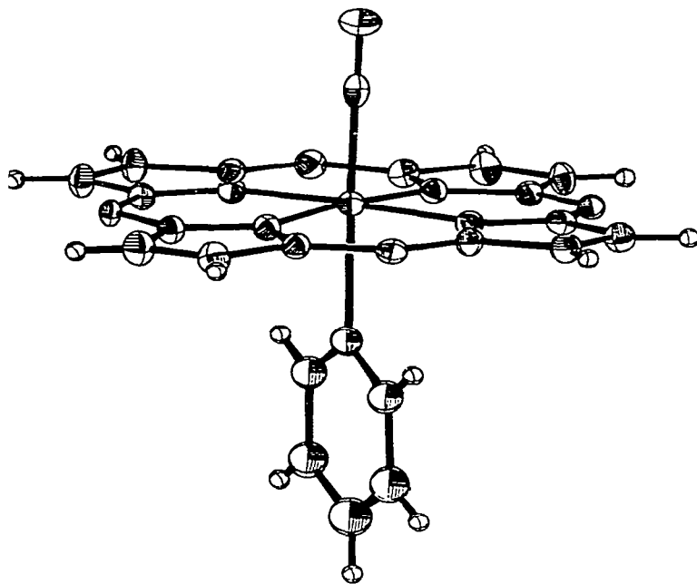
Fig. 3. Computer drawing of the molecule Ru(TPP)CO(Py) from ref. 13.
