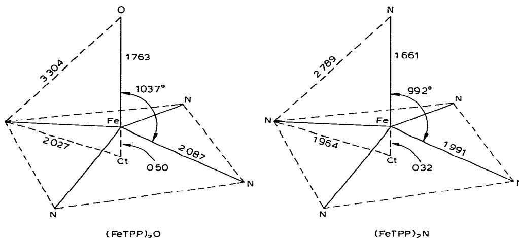
Fig. 25. Comparison of coordination geometries for [\text{Fe}(\text{TPP})]_2\text{O} and [\text{Fe}(\text{TPP})]_2\text{N} from ref. 50.
