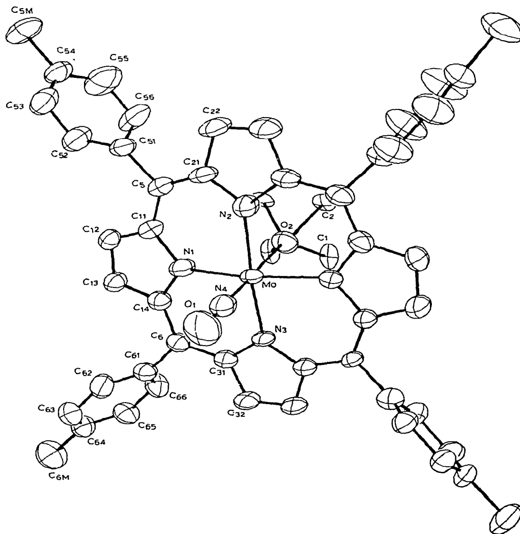
Fig. 13. Computer drawing of the molecule \text{Mo}(\text{TPP})\text{NO}(\text{MeOH}) from ref. 26.
