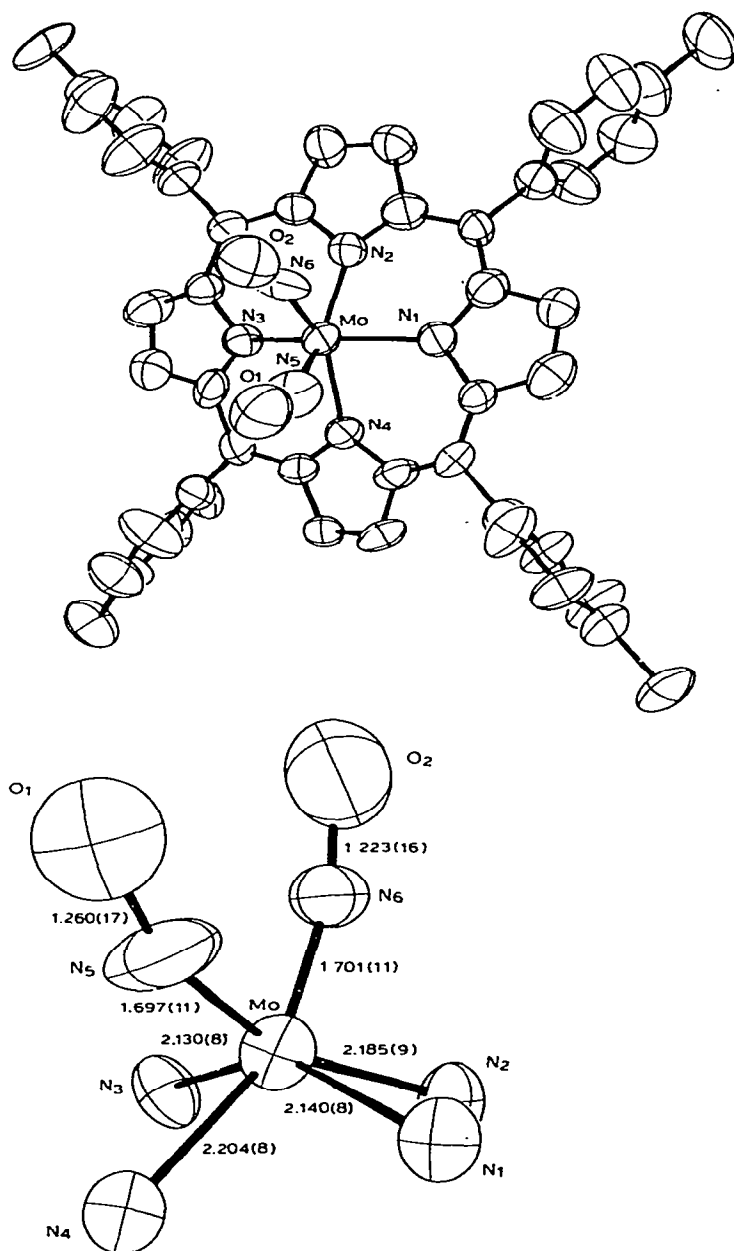
Fig. 15. Computer drawing and inner coordination sphere of the molecule \text{Mo(TPP)(NO)}_2 from ref. 26.
