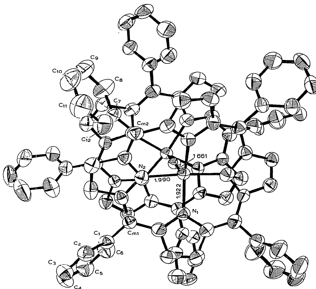
Fig. 24. Computer drawing of the molecule [\text{Fe}(\text{TPP})]_2\text{N} from ref. 160.
