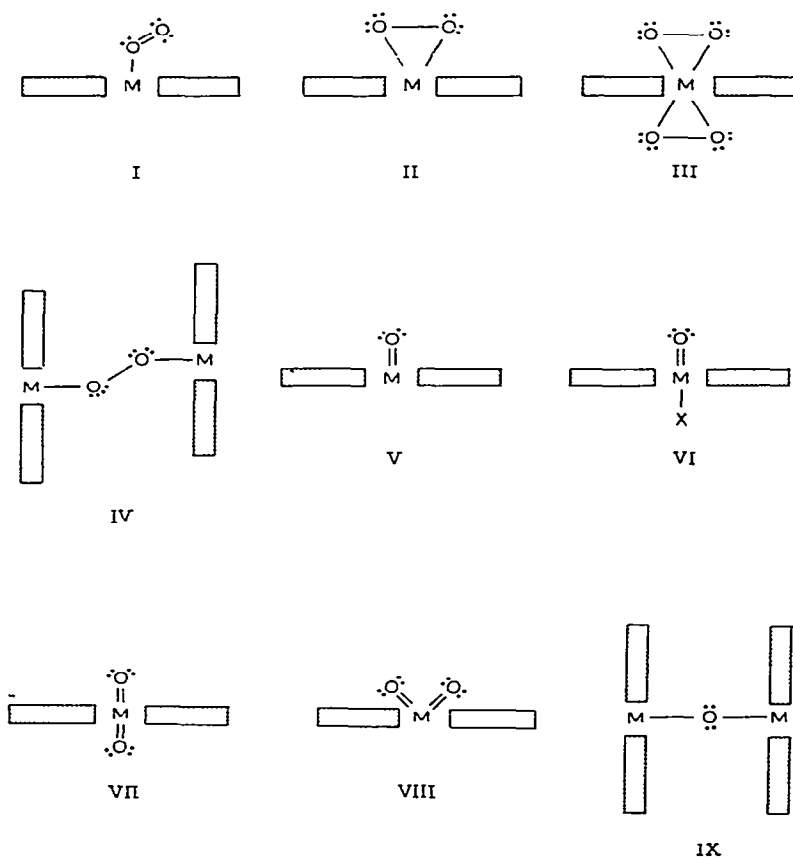
Fig. 16. Major types of metalloporphyrin oxygen complexes.
