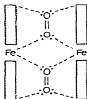
Fig. 17. Proposed structure, for the reversible 1:1 O 2 binding by solid four-coordinate hemes.
